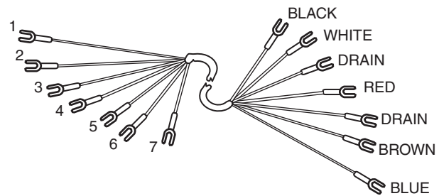
Figure 8. Extension Cable (Part 6000130)
