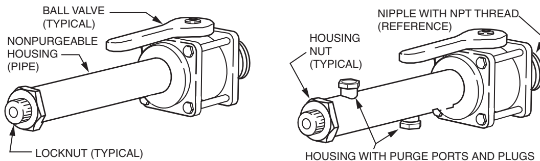
Figure 1. Typical Ball Valve Assemblies
