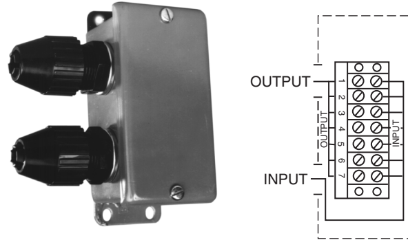
Figure 7. Extension Cable Assembly (Part 0060901)
