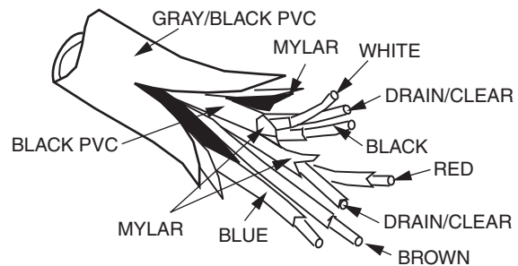
Figure 8. Extension Cable (Part 6000130)
