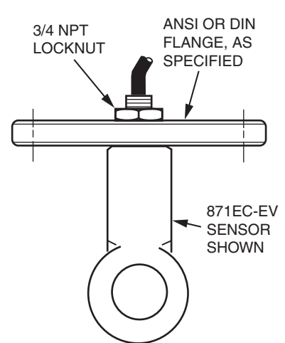
TYPICAL FLANGE MOUNTING CONFIGURATION
