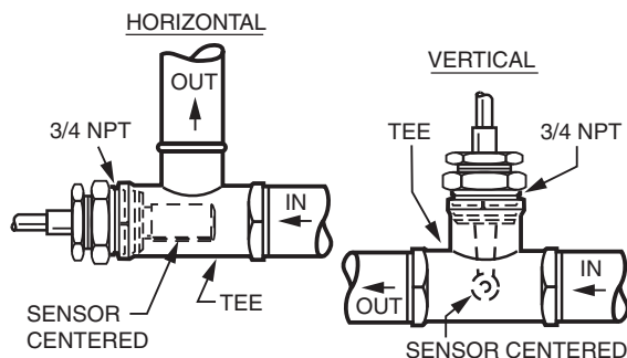
Figure 4. Tee Installations
